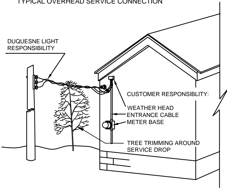
TYPICAL OVERHEAD SERVICE CONNECTION
