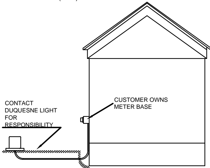
TYPICAL SERVICE IN UNDERGROUND RESIDENTIAL DEVELOPMENT (URD)
